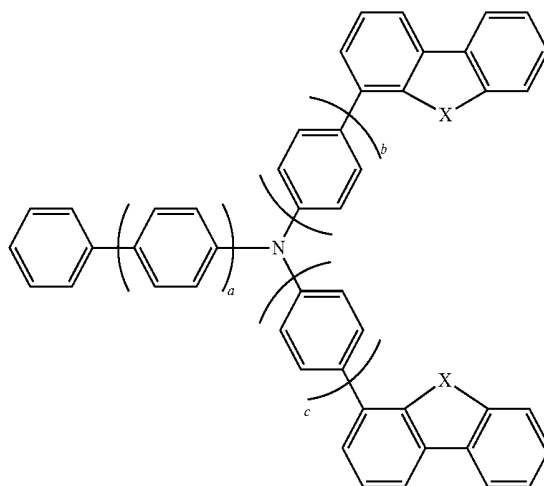
Chemical Formula 2
