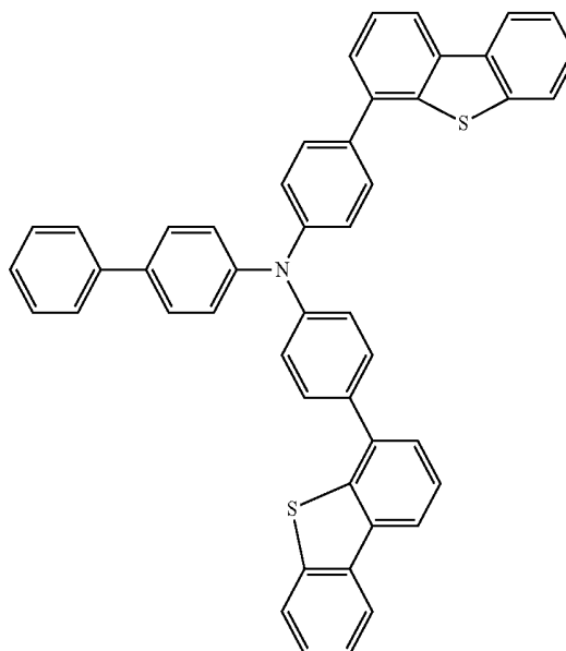
Chemical Formula 2-4
