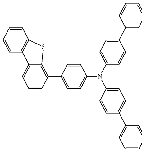
Chemical Formula 1-6
