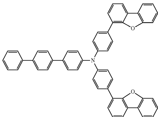
Chemical Formula 2-1
