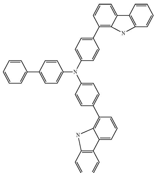
Chemical Formula 2-2
